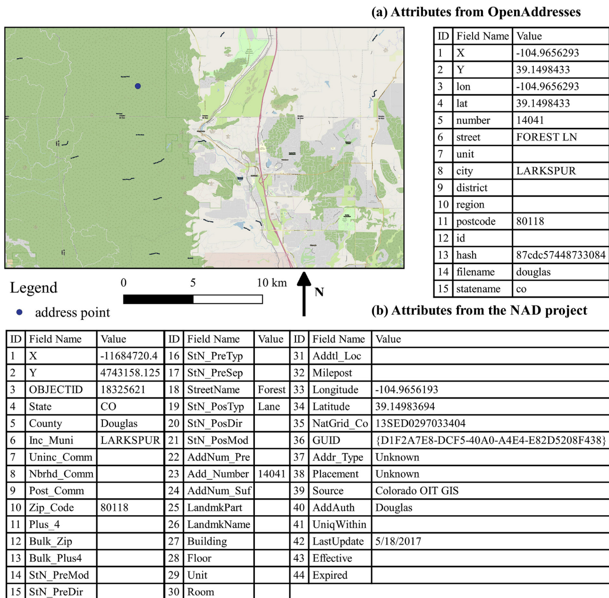
Fig. 1. An example of the address point data from the OpenAddresses and NAD project.
