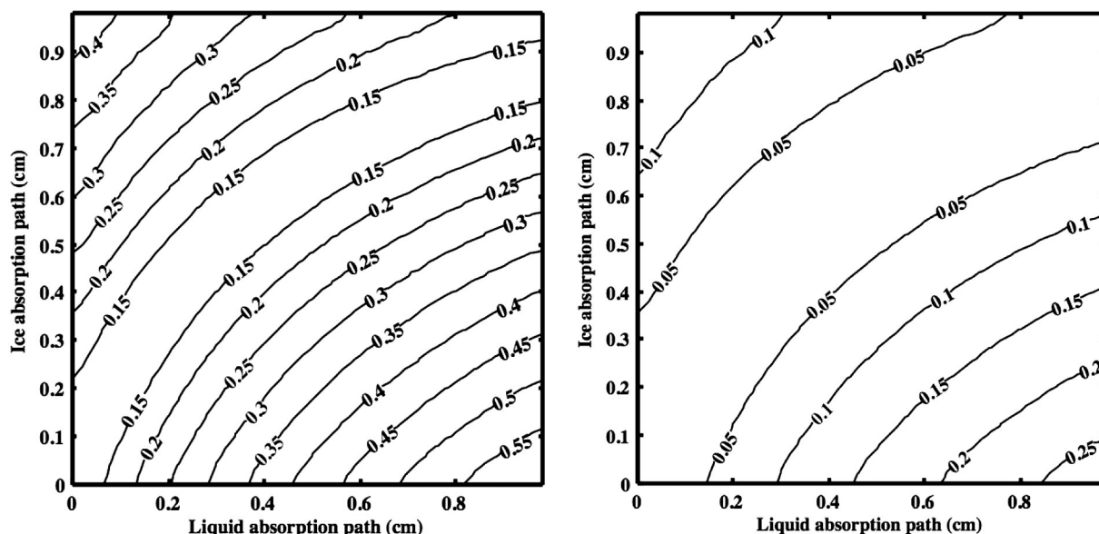
Fig. 3. Mean absolute errors in water vapor estimation (units of cm), over vapor paths from 0 to 2 cm. Axes show actual liquid and ice absorption paths. Left: Errors resulting from a band depth approach. Right: A simultaneous retrieval of three water phases improves accuracy.
