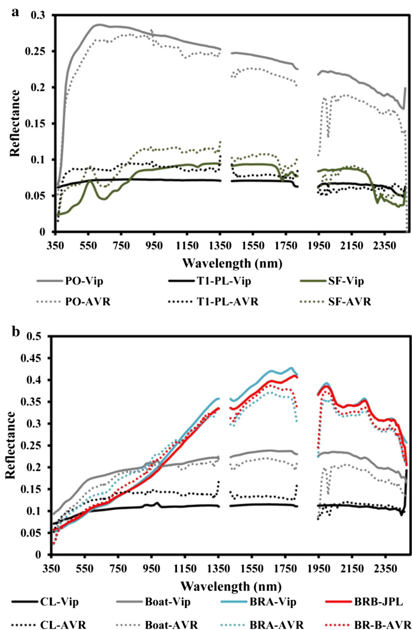
Fig. 9. ASD (solid) and AVIRIS-derived (dotted) reflectance measured along the southern (a) and northern (b) extents of the flight lines. Regions of strong water vapor absorption have been removed from field and AVIRIS reflectance spectra. Spectra include the Post Office Roof (PO), USDA Parking Lot (T1-PL), Soccer Field (SF), Church Parking Lot (CL), Boat Ramp (Boat), Bare Rock A and Bare Rock B (Table 1). The spectrum for the beach at Huntington Lake is not shown because it was snow-covered in April, 2014, but was included in the regression relationship for 2013. Vip refers to the approach in which a spectrum was collected every 4 m, JPL refers to a transect collected using continuous observations (see Methods).
