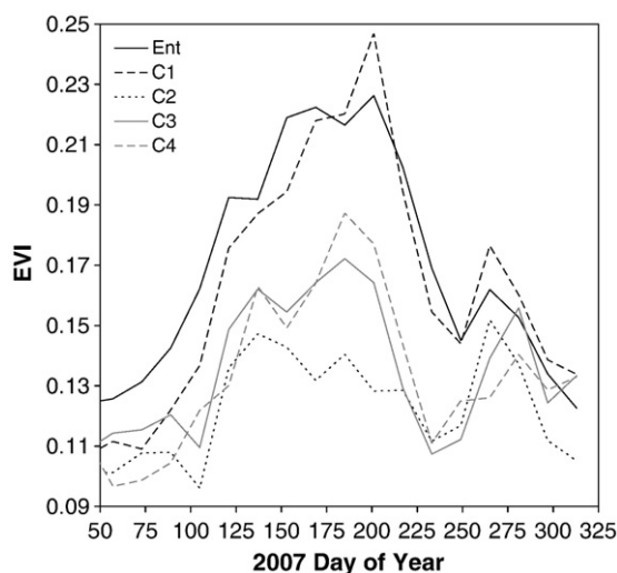
Fig. 6. Average EVI from 6–8 MODIS pixels for 5 different sites during mid-2007.
