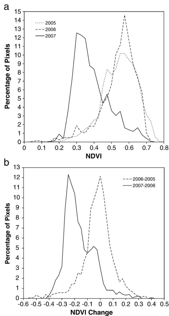
Fig. 4. a) Histograms of NDVI values for all pixels within the tamarisk polygons, extracted from the 2005, 2006, and 2007 ASTER images. b) Histograms of change in NDVI between two ASTER image dates. A negative change indicates a drop in NDVI between the earlier and later image.
