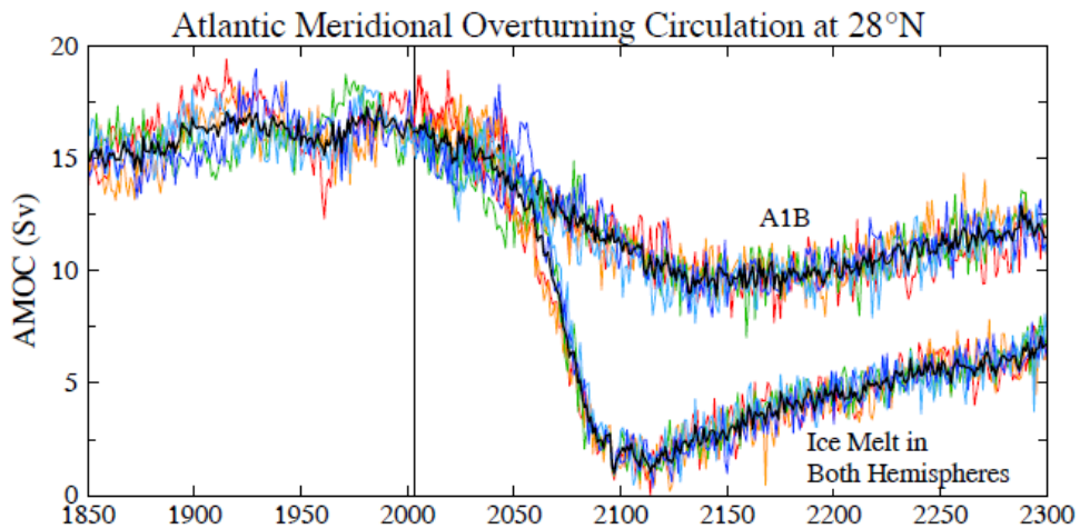
Fig. S9. AMOC strength at 28^{\circ}\text{N} in five ensemble members and their mean (heavy black line) for the A1B GHG scenario and for that scenario plus ice melt in both hemispheres with 10-year doubling time reaching a maximum 5 m contribution to sea level.
