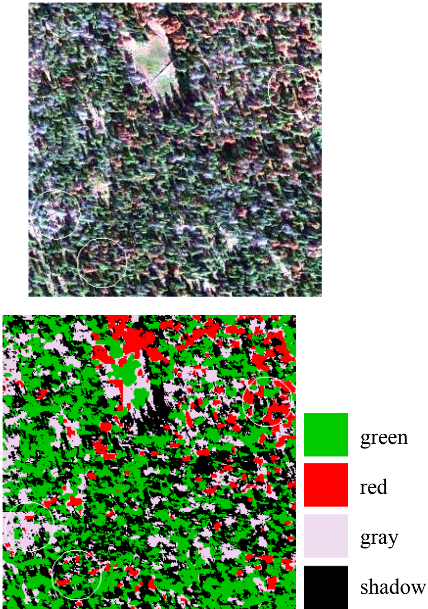
Figure 2. The top image is a 150m by 150 m subset, true-color composite of the pan-sharpened GeoEye-1 data. The bottom image is the maximum likelihood classification of the same area shown in the top image. The locations of three 12.62 m radius plots (circles) are shown in each image. Plot 2 is adjacent to the left edge of the image, plot 12 is adjacent to the bottom edge of the image, and plot 3 is adjacent to the right edge of the image.
