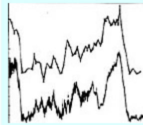
CO 2 & temperature
