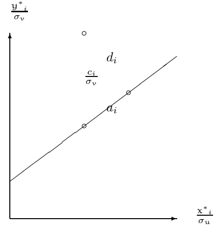
FIGURE 11. Geometric Interpretation of Objective Function
